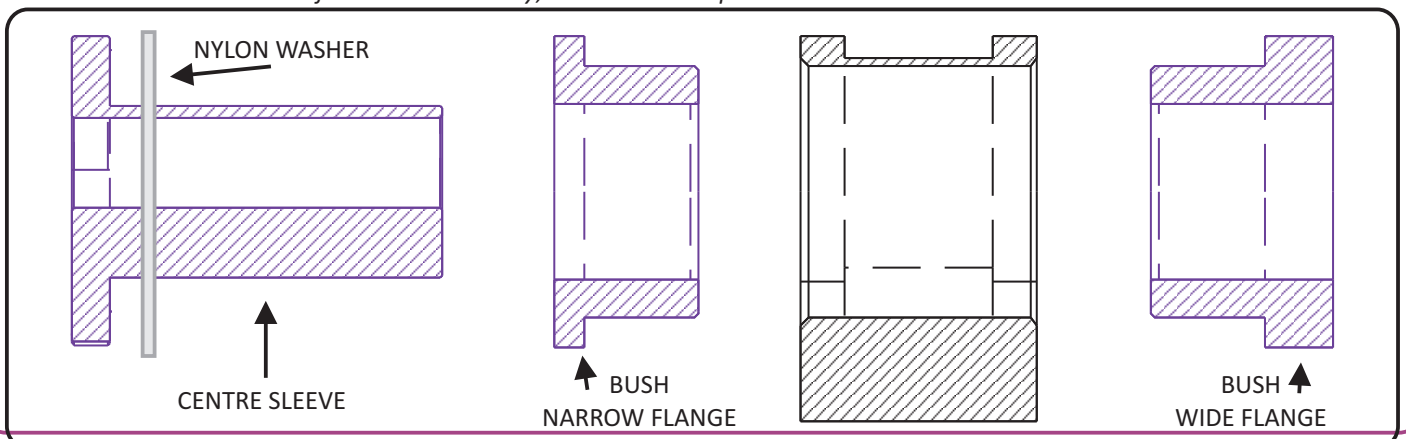
Fig 3. Exploded view.
