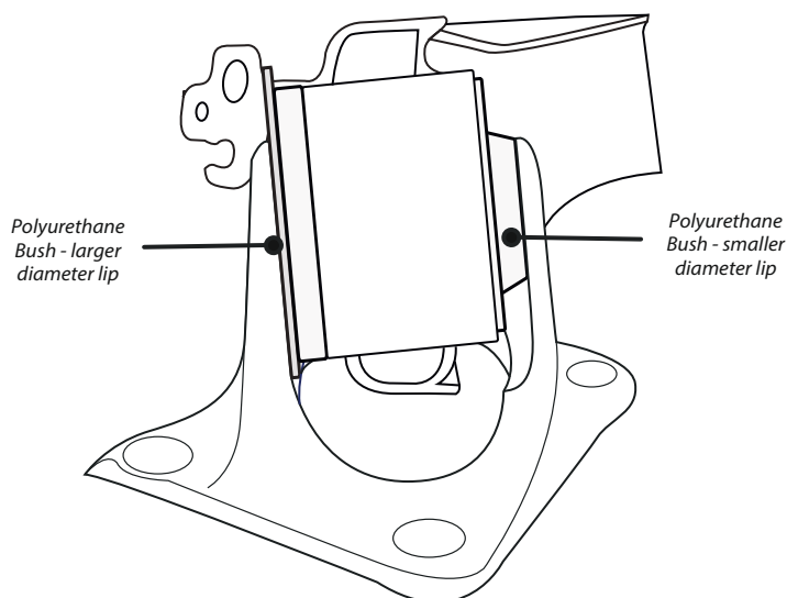
Figure 1 - diagram showing how the bush will fit inside the rear beam mount
