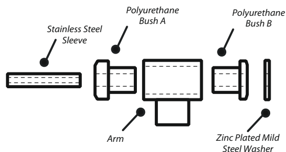
Figure 2 - Assembly
