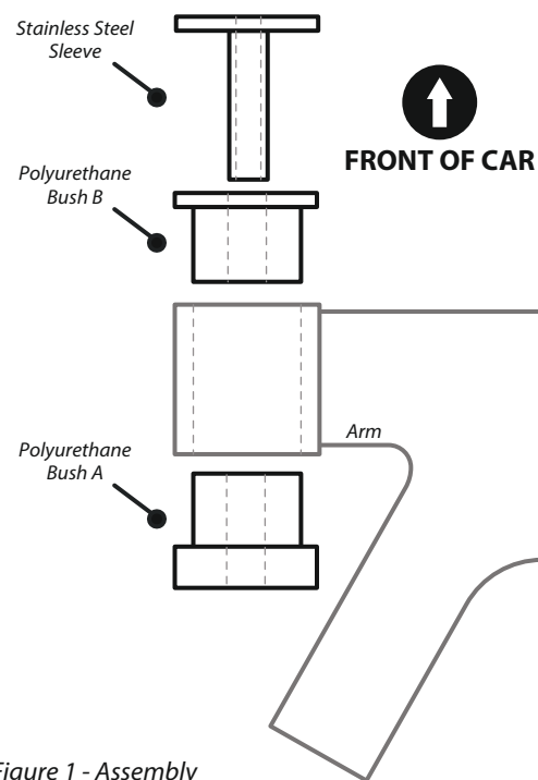
Figure 1 - Assembly
