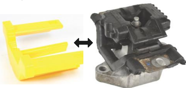
Figure 2 - exploded view showing how part A insert fits inside the gearbox mount
